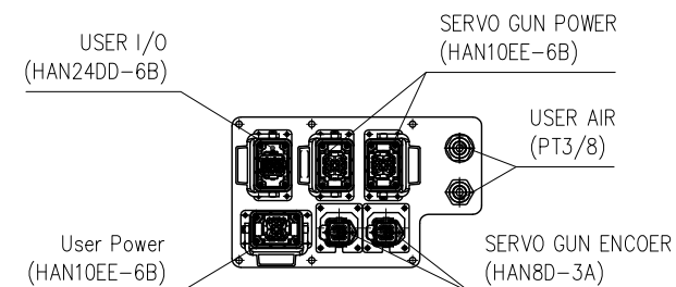
VIEW "D"
