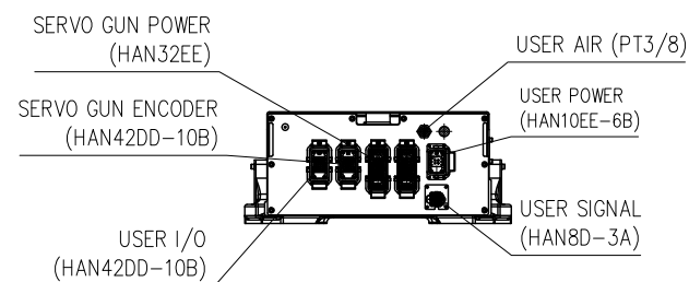
VIEW "C"
